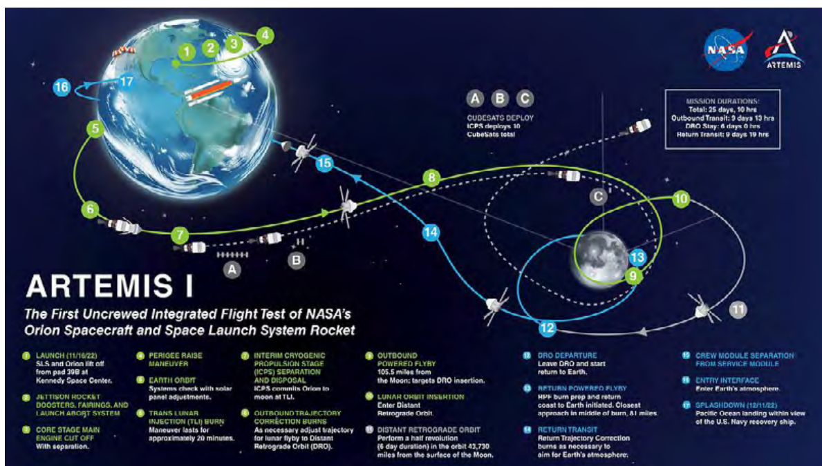
Figure 1. Artemis 1 trajectory map © NASA
